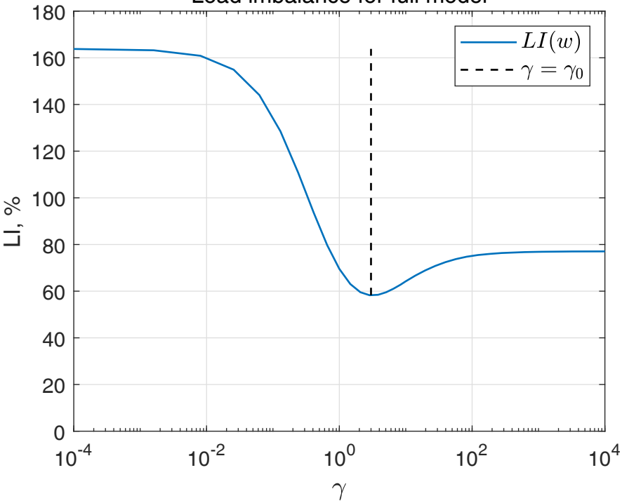
Load imbalance for full model
