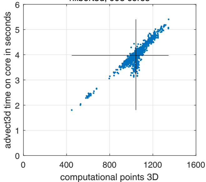
hilbert3d, 993 cores
