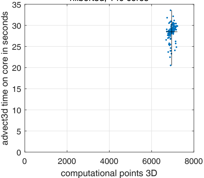
hilbert3d, 149 cores
