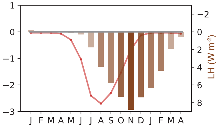
(e) Canopy transpiration change
