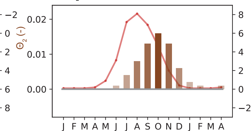
(h) \Theta_2 change
