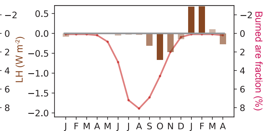
(f) Soil evaporation change
