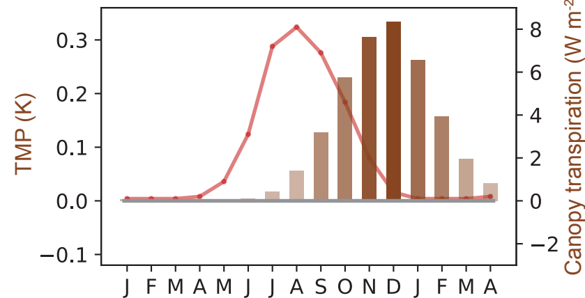
(g) \Theta_1 change
