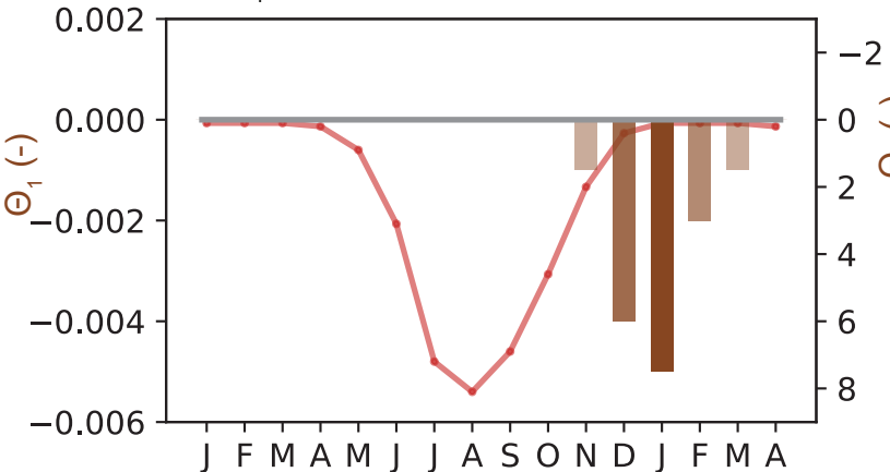
(g) \Theta_1 change
