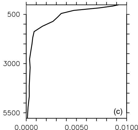
Seafloor Flux ( \text{Tmol Si m}^{-1} \text{yr}^{-1} )
