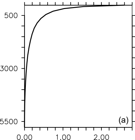
Opal Export ( \text{Tmol Si m}^{-1} \text{yr}^{-1} )
