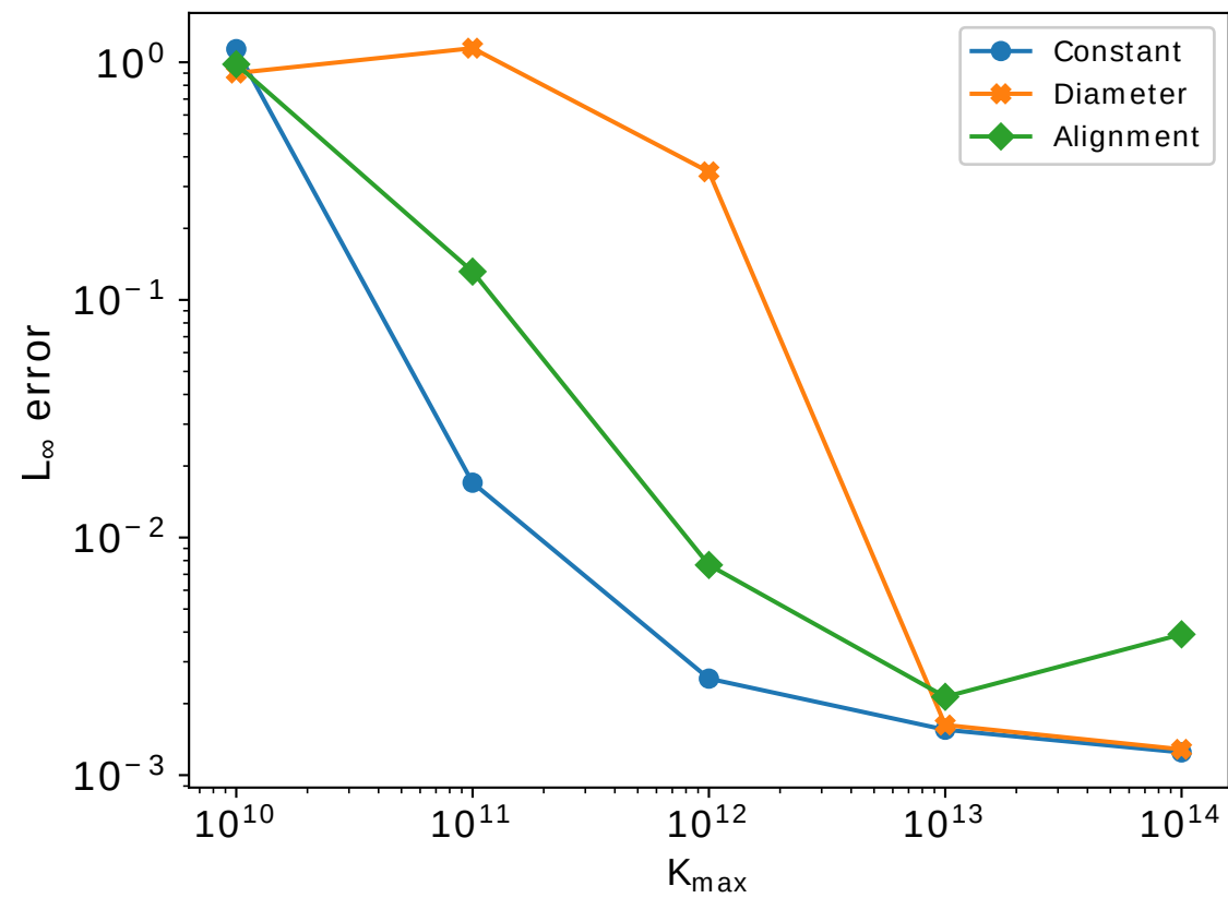
TC2: L_\infty u errors
