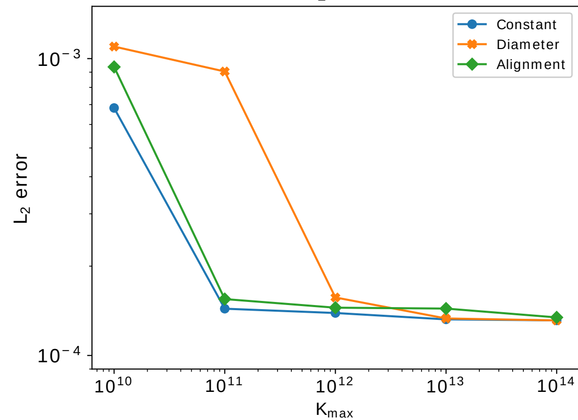
TC2: L_2 h errors
