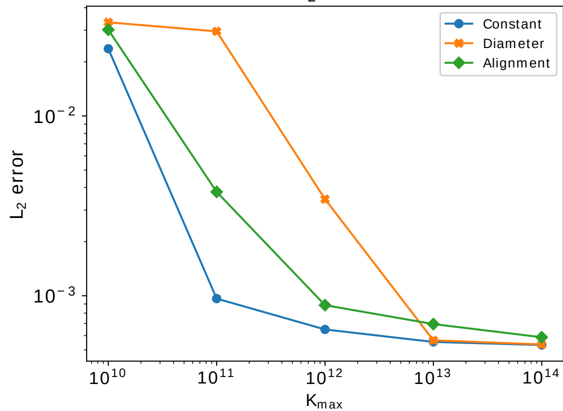
TC2: L_2 u errors
