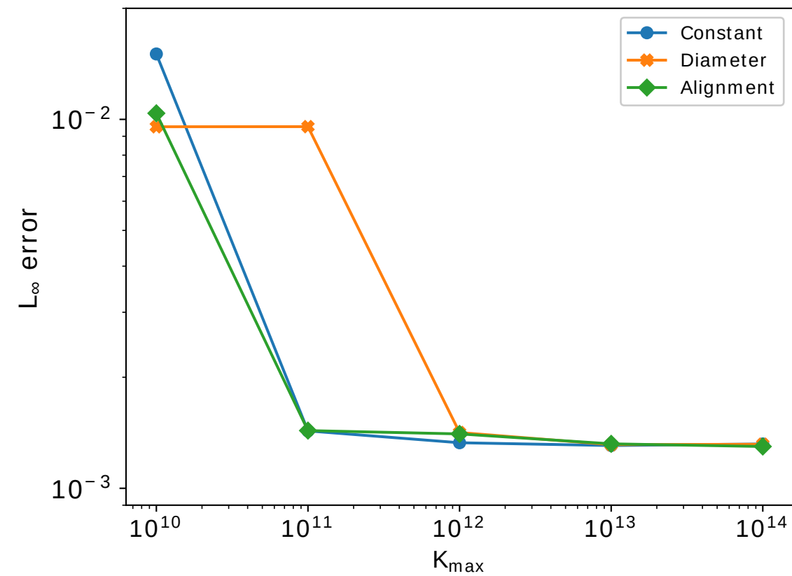
TC2: L_\infty h errors
