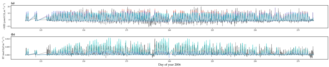
Figure S1. Comparison of model predicted carbon/water fluxes to US-NR1 (Niwot Ridge, evergreen gymnosperm forest) flux tower observations for year 2006. (a) Gray curve plots the half-hourly net ecosystem exchange ( \text{CO}_2 flux; NEE) in the growing season. Shaded red, blue, and cyan curve each plots the Ball et al. (1987), Medlyn et al. (2011), and Wang et al. (2020) stomatal model predictions (BBM, MED, and OSM), respectively. (b) Comparison of modeled and observed half-hourly total transpiration flux (water flux; ET).
