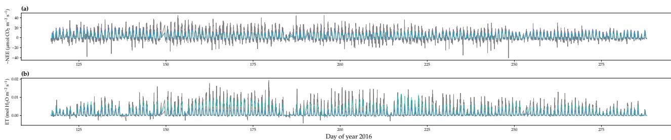
Figure S23. Comparison of model predicted carbon/water fluxes to US-MOz (Ozark, deciduous angiosperm forest) flux tower observations for year 2016. (a) Gray curve plots the half-hourly net ecosystem exchange ( \text{CO}_2 flux; NEE) in the growing season. Shaded red, blue, and cyan curve each plots the Ball et al. (1987), Medlyn et al. (2011), and Wang et al. (2020) stomatal model predictions (BBM, MED, and OSM), respectively. (b) Comparison of modeled and observed half-hourly total transpiration flux (water flux; ET).
