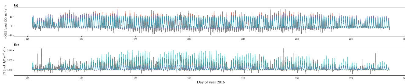
Figure S11. Comparison of model predicted carbon/water fluxes to US-NR1 (Niwot Ridge, evergreen gymnosperm forest) flux tower observations for year 2016. (a) Gray curve plots the half-hourly net ecosystem exchange ( \text{CO}_2 flux; NEE) in the growing season. Shaded red, blue, and cyan curve each plots the Ball et al. (1987), Medlyn et al. (2011), and Wang et al. (2020) stomatal model predictions (BBM, MED, and OSM), respectively. (b) Comparison of modeled and observed half-hourly total transpiration flux (water flux; ET).
