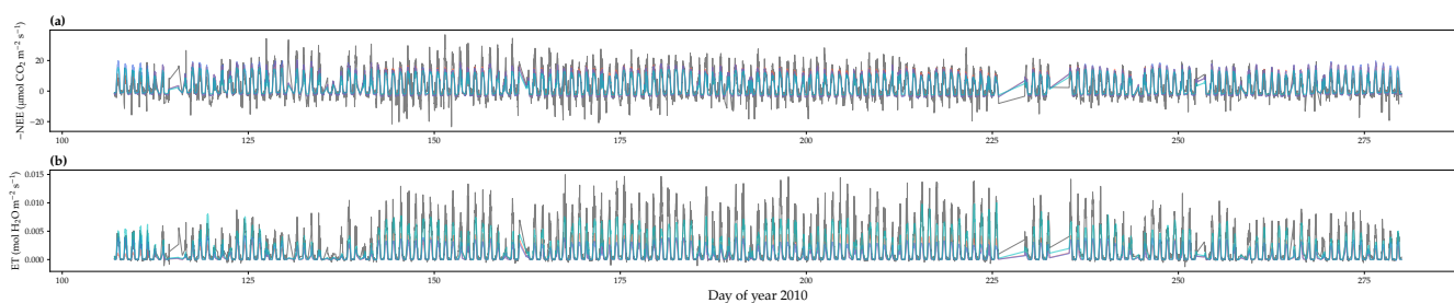
Figure S18. Comparison of model predicted carbon/water fluxes to US-MOz (Ozark, deciduous angiosperm forest) flux tower observations for year 2010. (a) Gray curve plots the half-hourly net ecosystem exchange ( \text{CO}_2 flux; NEE) in the growing season. Shaded red, blue, and cyan curve each plots the Ball et al. (1987), Medlyn et al. (2011), and Wang et al. (2020) stomatal model predictions (BBM, MED, and OSM), respectively. (b) Comparison of modeled and observed half-hourly total transpiration flux (water flux; ET).
