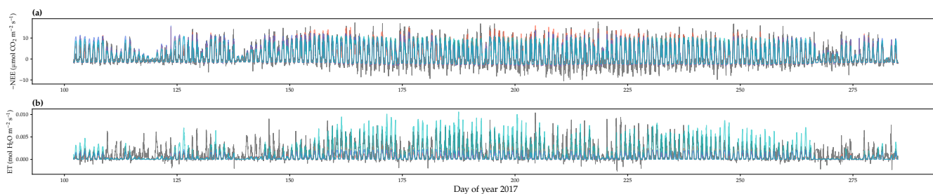
Figure S12. Comparison of model predicted carbon/water fluxes to US-NR1 (Niwot Ridge, evergreen gymnosperm forest) flux tower observations for year 2017. (a) Gray curve plots the half-hourly net ecosystem exchange ( \text{CO}_2 flux; NEE) in the growing season. Shaded red, blue, and cyan curve each plots the Ball et al. (1987), Medlyn et al. (2011), and Wang et al. (2020) stomatal model predictions (BBM, MED, and OSM), respectively. (b) Comparison of modeled and observed half-hourly total transpiration flux (water flux; ET).
