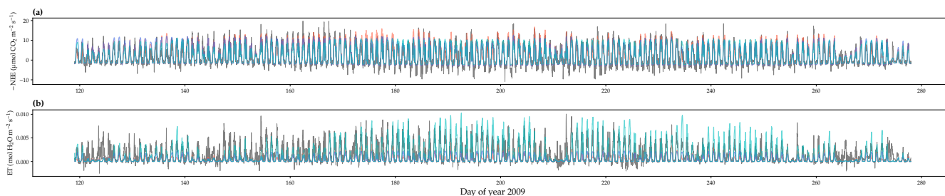
Figure S4. Comparison of model predicted carbon/water fluxes to US-NR1 (Niwot Ridge, evergreen gymnosperm forest) flux tower observations for year 2009. (a) Gray curve plots the half-hourly net ecosystem exchange ( \text{CO}_2 flux; NEE) in the growing season. Shaded red, blue, and cyan curve each plots the Ball et al. (1987), Medlyn et al. (2011), and Wang et al. (2020) stomatal model predictions (BBM, MED, and OSM), respectively. (b) Comparison of modeled and observed half-hourly total transpiration flux (water flux; ET).
