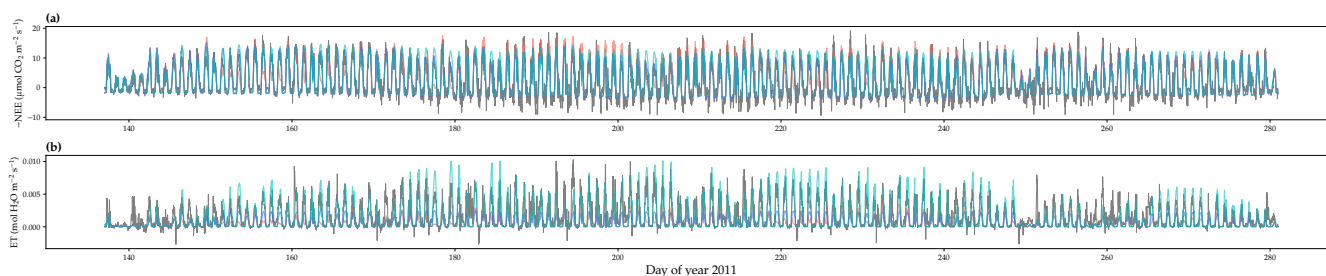
Figure S6. Comparison of model predicted carbon/water fluxes to US-NR1 (Niwot Ridge, evergreen gymnosperm forest) flux tower observations for year 2011. (a) Gray curve plots the half-hourly net ecosystem exchange ( \text{CO}_2 flux; NEE) in the growing season. Shaded red, blue, and cyan curve each plots the Ball et al. (1987), Medlyn et al. (2011), and Wang et al. (2020) stomatal model predictions (BBM, MED, and OSM), respectively. (b) Comparison of modeled and observed half-hourly total transpiration flux (water flux; ET).
