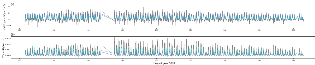
Figure S17. Comparison of model predicted carbon/water fluxes to US-MOz (Ozark, deciduous angiosperm forest) flux tower observations for year 2009. (a) Gray curve plots the half-hourly net ecosystem exchange ( \text{CO}_2 flux; NEE) in the growing season. Shaded red, blue, and cyan curve each plots the Ball et al. (1987), Medlyn et al. (2011), and Wang et al. (2020) stomatal model predictions (BBM, MED, and OSM), respectively. (b) Comparison of modeled and observed half-hourly total transpiration flux (water flux; ET).
