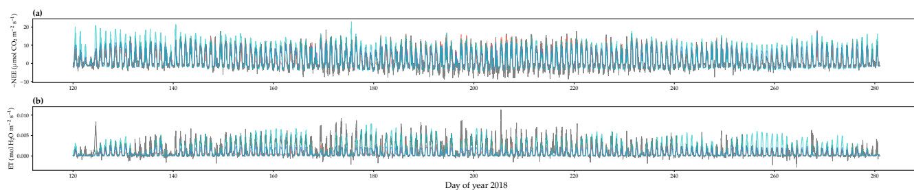
Figure S13. Comparison of model predicted carbon/water fluxes to US-NR1 (Niwot Ridge, evergreen gymnosperm forest) flux tower observations for year 2018. (a) Gray curve plots the half-hourly net ecosystem exchange ( \text{CO}_2 flux; NEE) in the growing season. Shaded red, blue, and cyan curve each plots the Ball et al. (1987), Medlyn et al. (2011), and Wang et al. (2020) stomatal model predictions (BBM, MED, and OSM), respectively. (b) Comparison of modeled and observed half-hourly total transpiration flux (water flux; ET).
