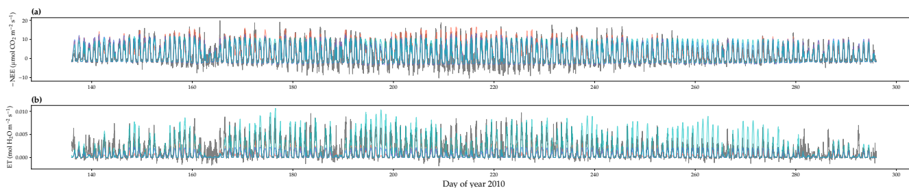
Figure S5. Comparison of model predicted carbon/water fluxes to US-NR1 (Niwot Ridge, evergreen gymnosperm forest) flux tower observations for year 2010. (a) Gray curve plots the half-hourly net ecosystem exchange ( \text{CO}_2 flux; NEE) in the growing season. Shaded red, blue, and cyan curve each plots the Ball et al. (1987), Medlyn et al. (2011), and Wang et al. (2020) stomatal model predictions (BBM, MED, and OSM), respectively. (b) Comparison of modeled and observed half-hourly total transpiration flux (water flux; ET).
