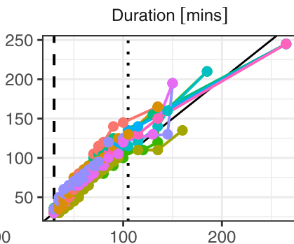
(h) WRF + TITAN (Thompson)
