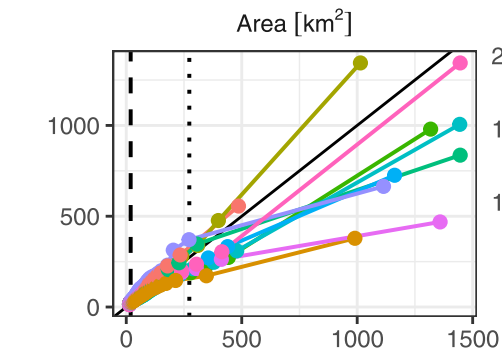
(g) WRF + TITAN (Thompson)
