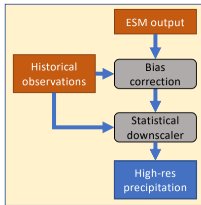
Statistical downscaling
