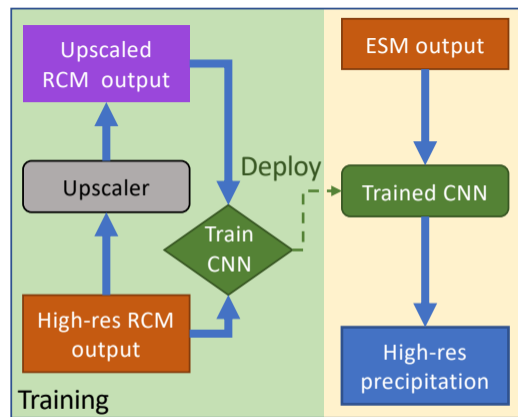
Super-resolution downscaling
