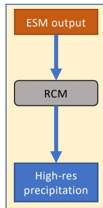
Dynamical downscaling
