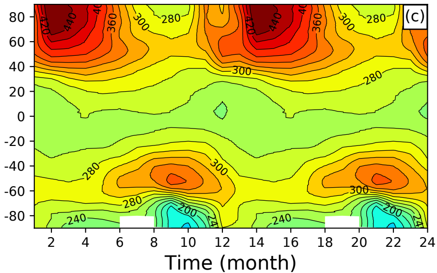
MSRv2
