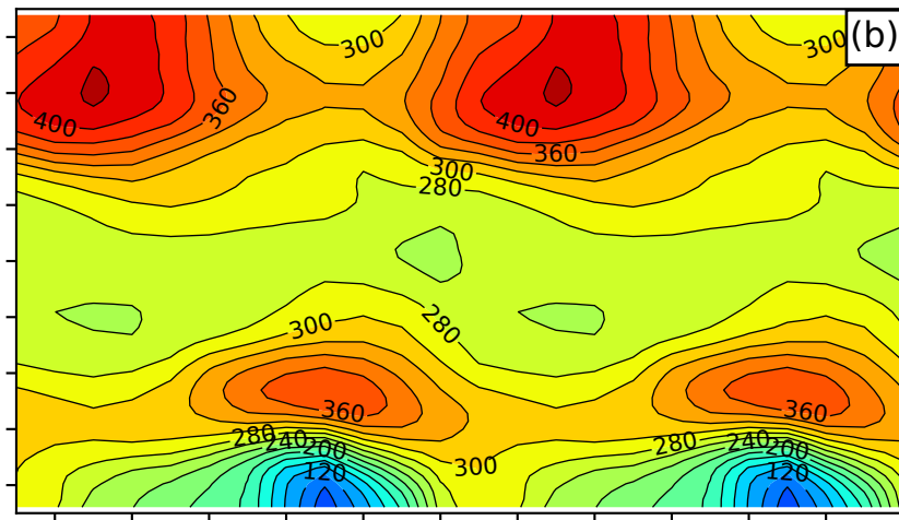
SOCOLv3
