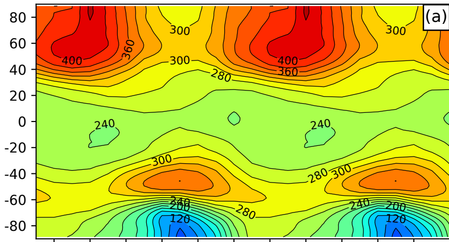
SOCOLv4
