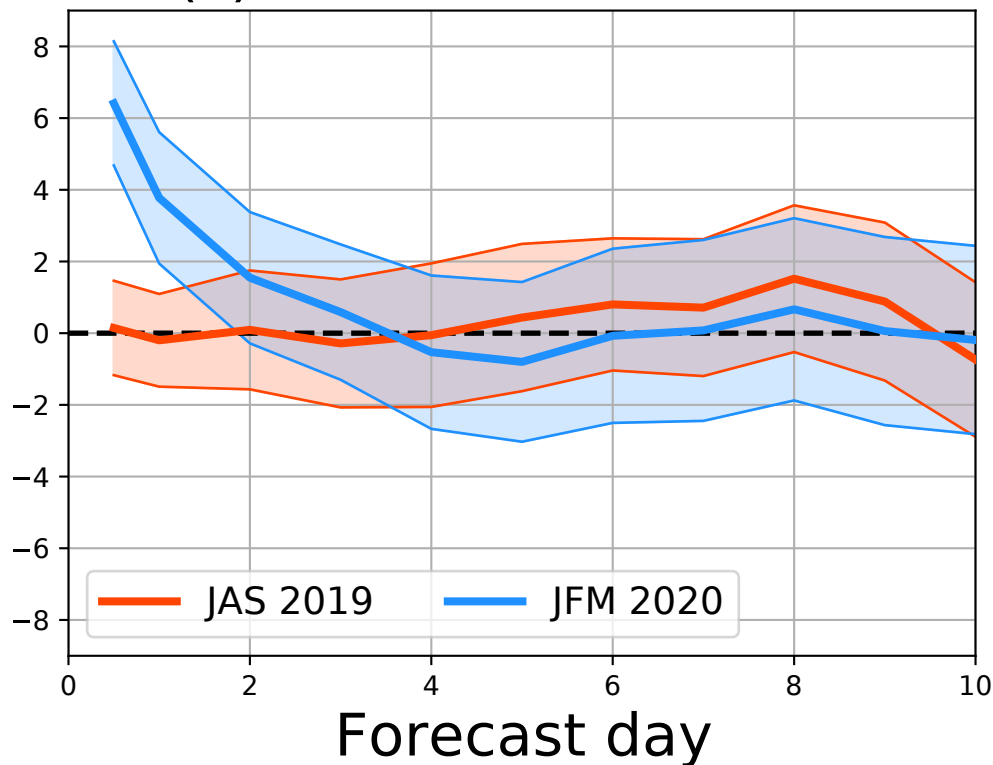
(c) Z: Antarctic 500 hPa
