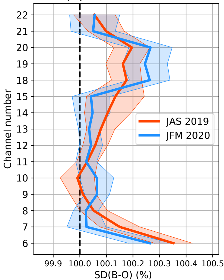
(a) ATMS - Global
