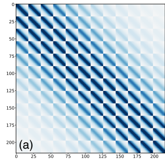
Prior
