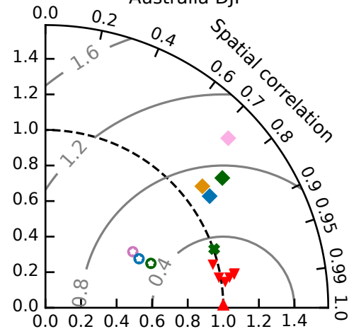
Australia DJF
