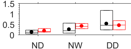
HCOOH
