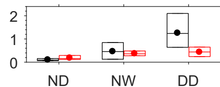
HCOOH
