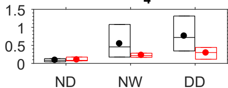
ISOPOOH/IEPOX
