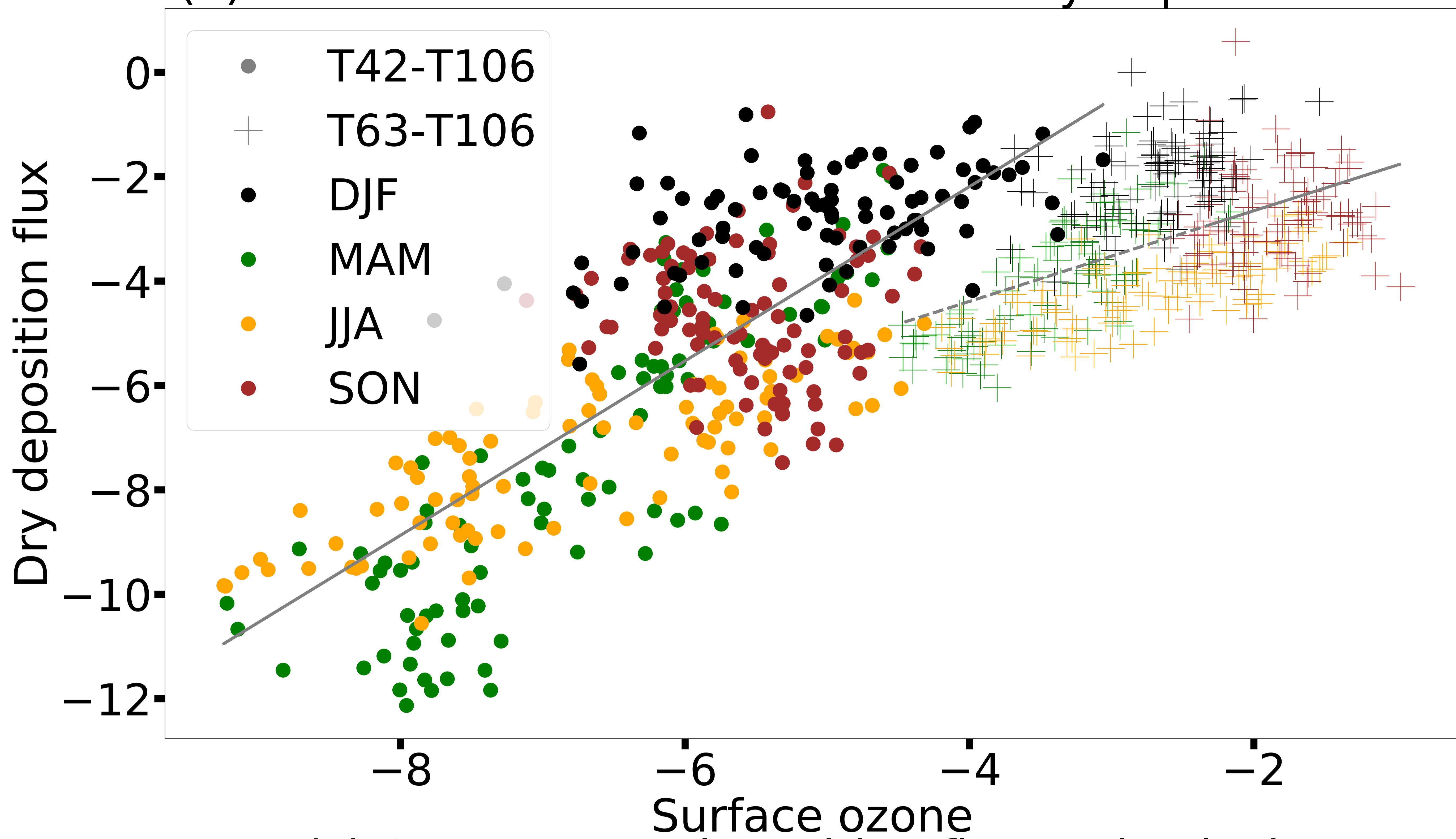
(c) SH_exT: Dry deposition flux and velocity
