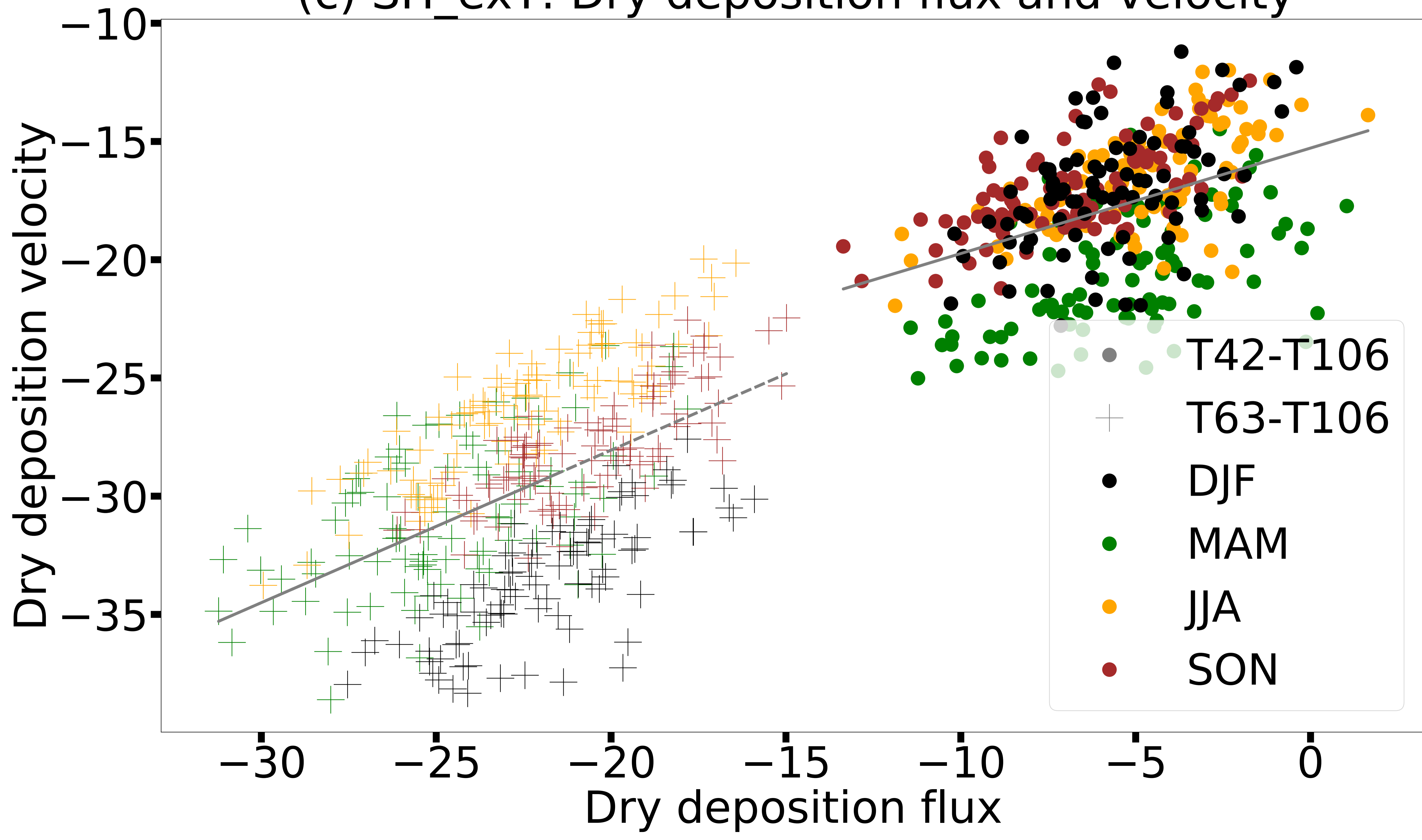
(c) SH_exT: Dry deposition flux and velocity
