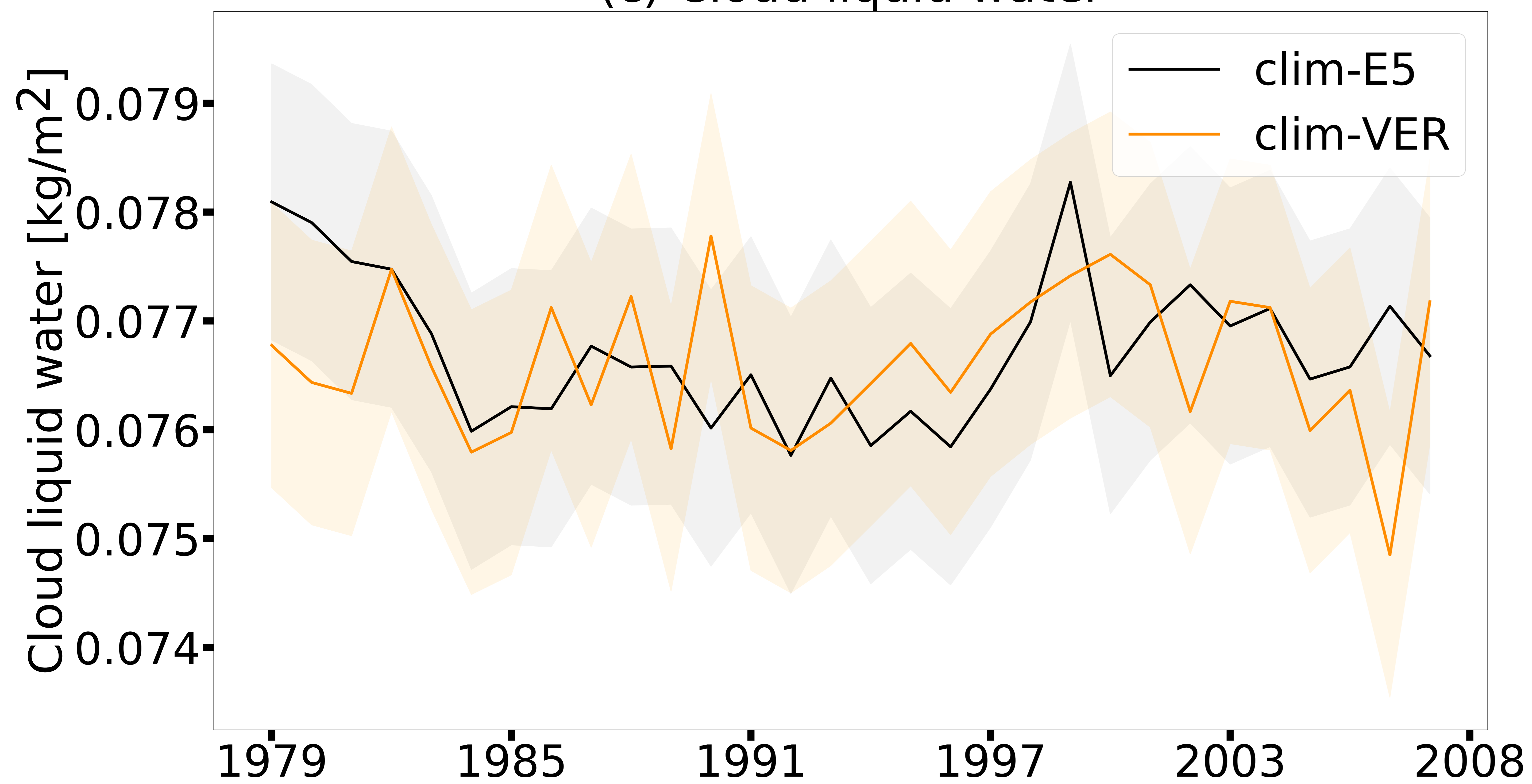
(c) Cloud liquid water
