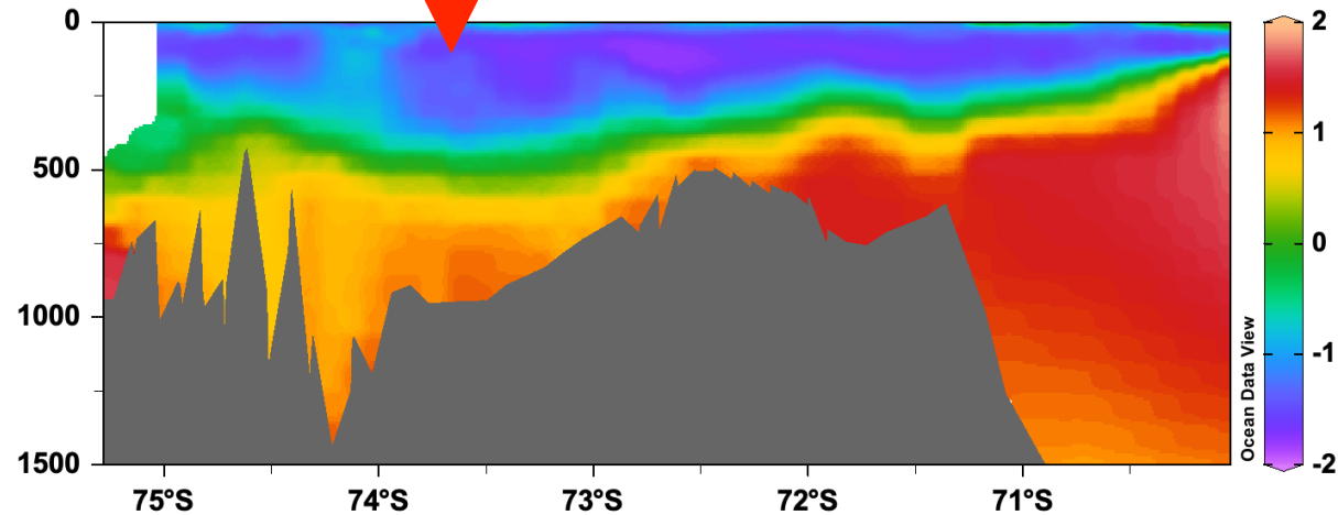
(b) 2014 Pot. Temp., iter20
