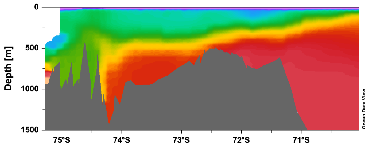
(c) 2014 Salinity, iter0
