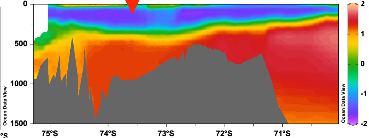
(b) 2010 Pot. Temp., iter20
