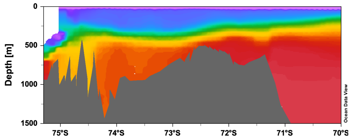
(c) 2010 Salinity, iter0
