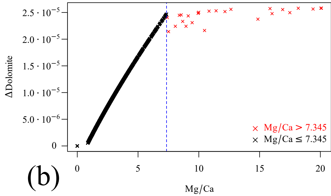
\Delta\text{Dolomite} vs. \text{Mg}/\text{Ca}
