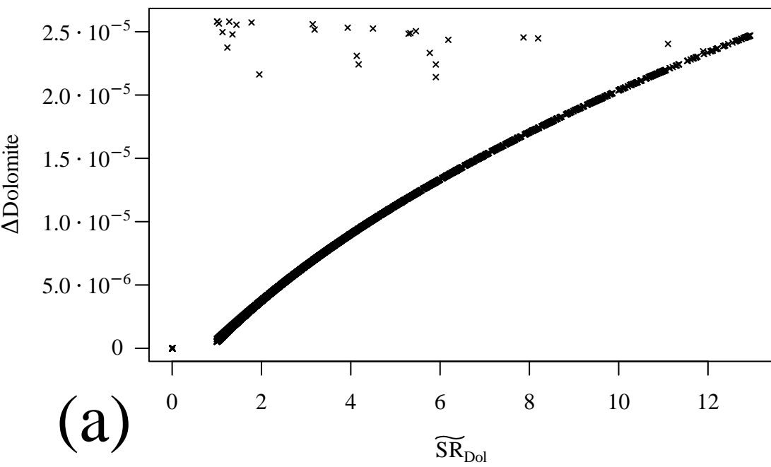
\Delta\text{Dolomite} vs. \widetilde{\text{SR}}_{\text{Dol}}
