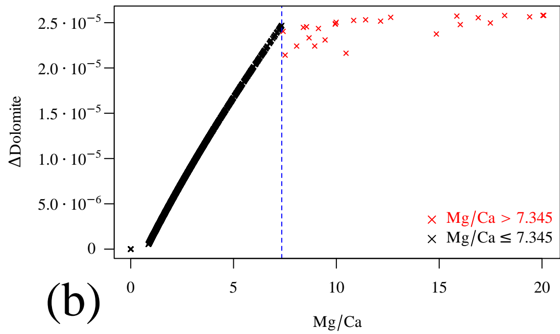
\Delta\text{Dolomite} vs. Mg/Ca
