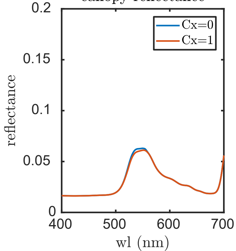
canopy reflectance
