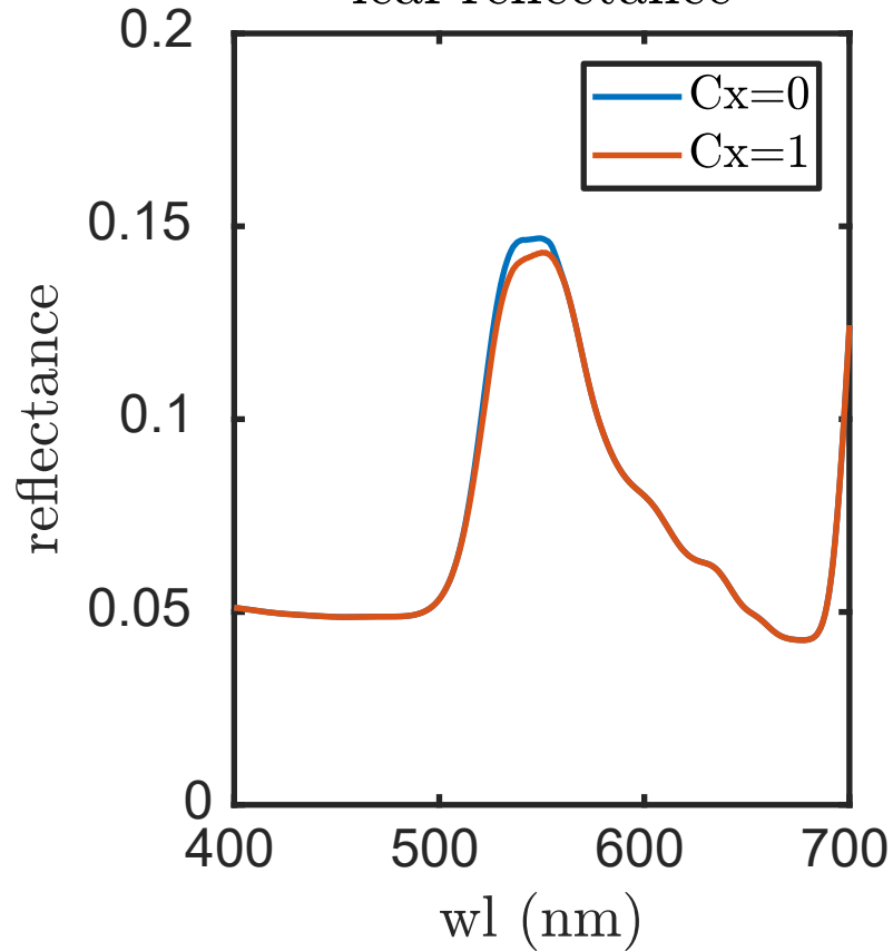
leaf reflectance
