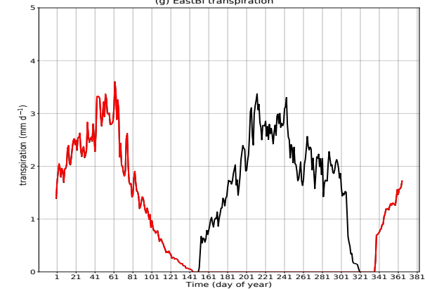
(g) EastBi transpiration
