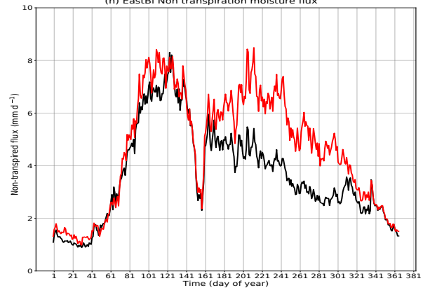
(h) EastBi Non transpiration moisture flux
