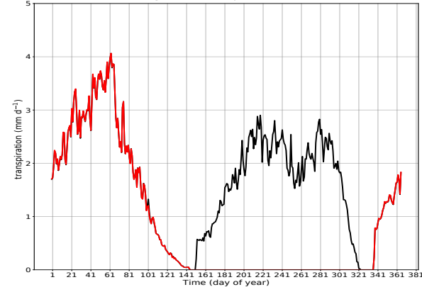
(g) EastUP transpiration
