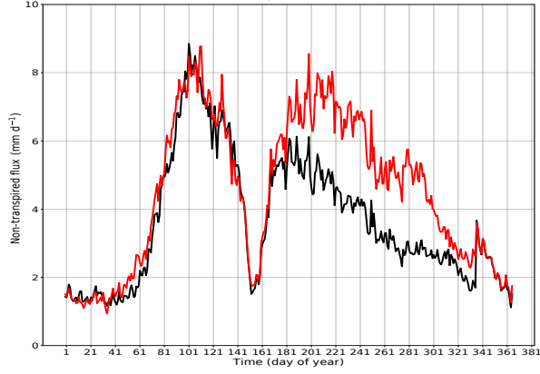
(h) EastUP Non transpiration moisture flux
