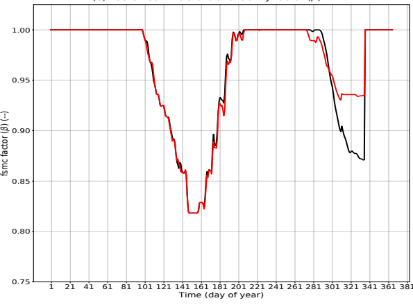
(g) EastUP transpiration
