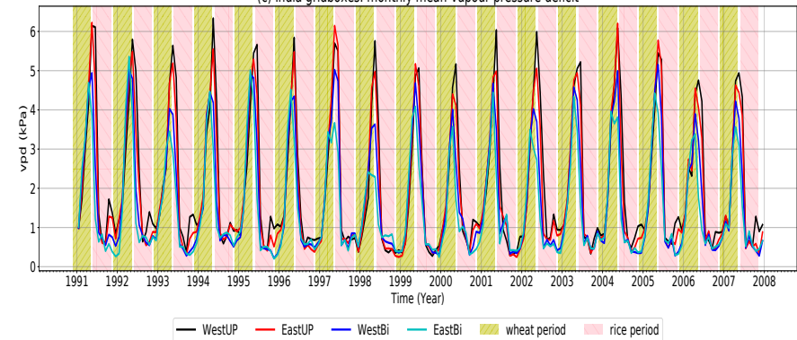
(c) India gridboxes: monthly mean Vapour pressure deficit
