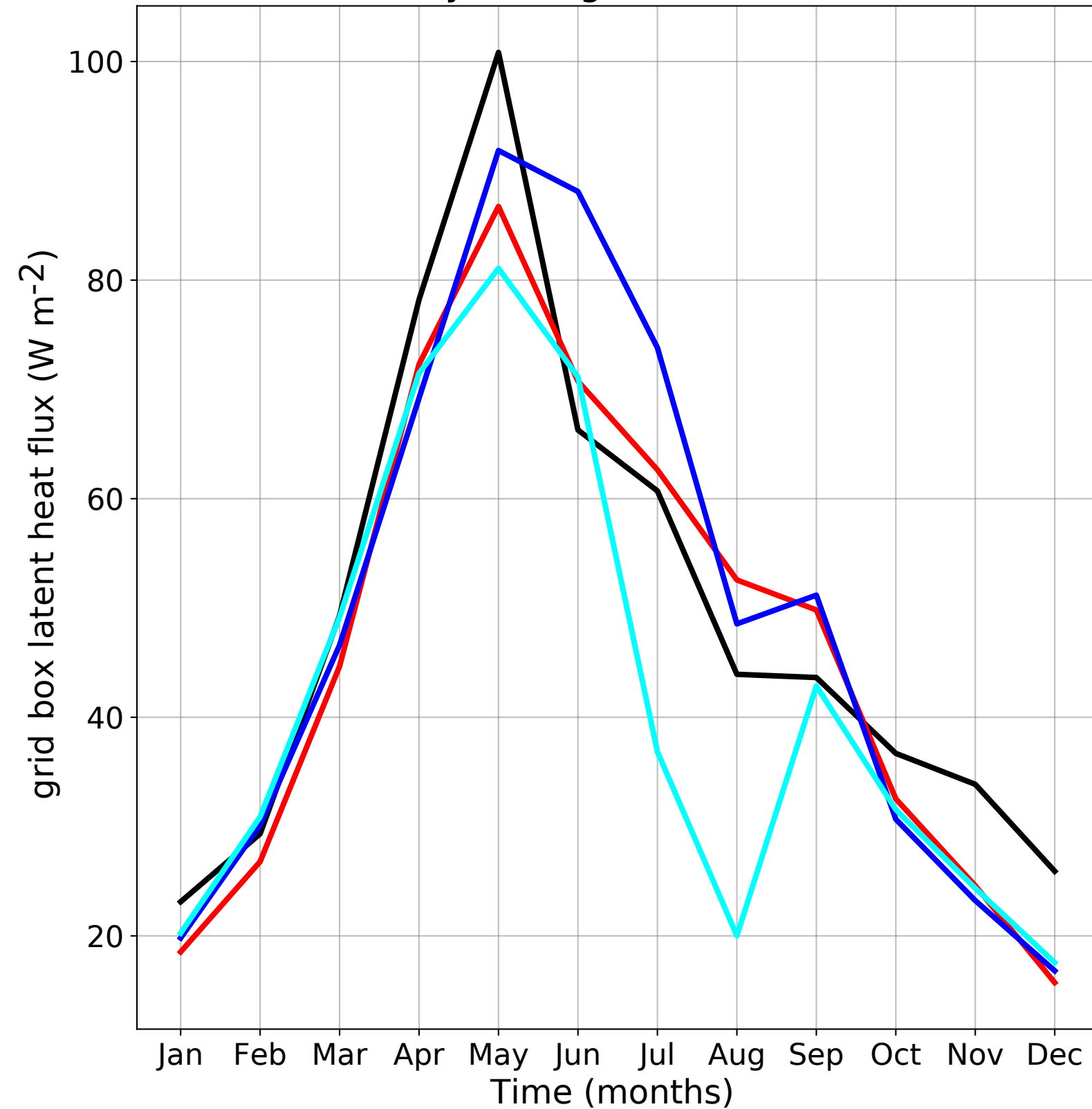
(b) Annual cycle of grid box latent heat flux
