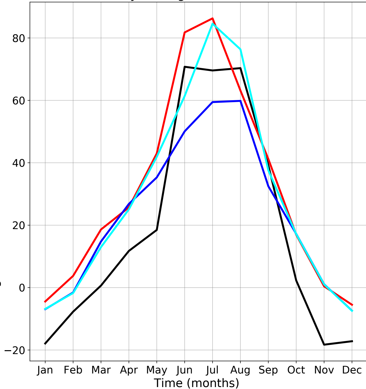
(a) Annual cycle of grid box sensible heat flux
