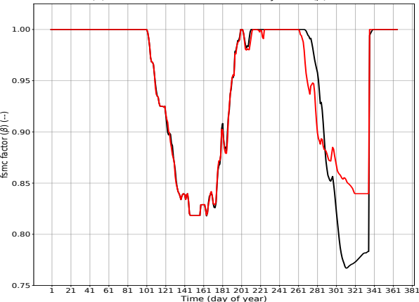
(g) WestUP transpiration
