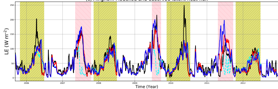
(c) Avignon: Modelled and observed latent heat flux
