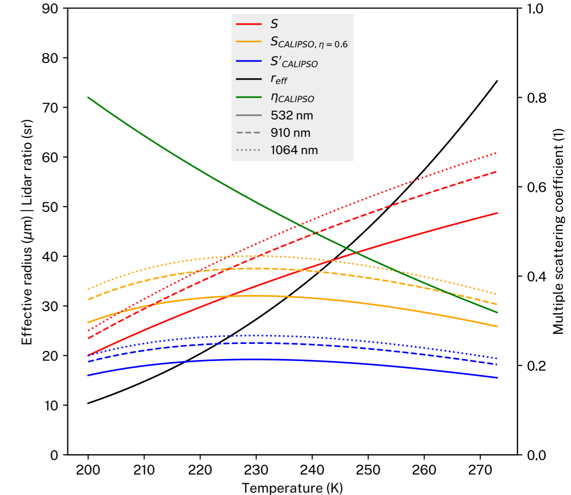
(c) Ice cloud optical parameters
