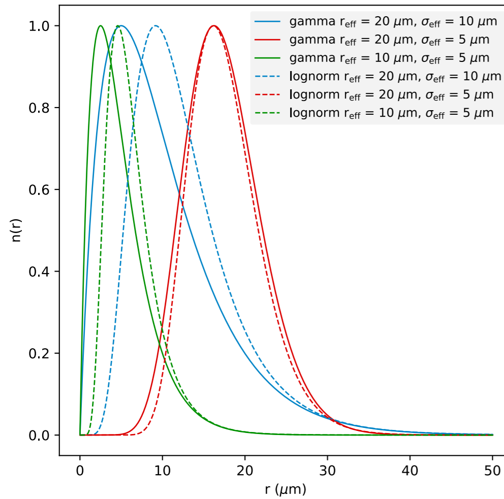
(a) Size distribution
