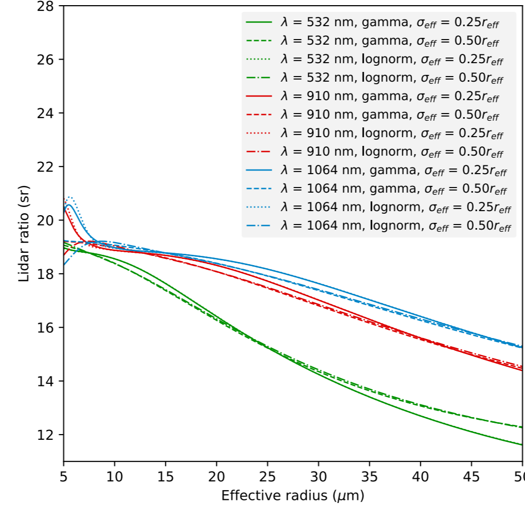
(b) Lidar ratio
