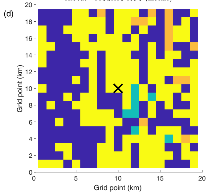
Albedo - MOSAIC-RUC (mosaic)
