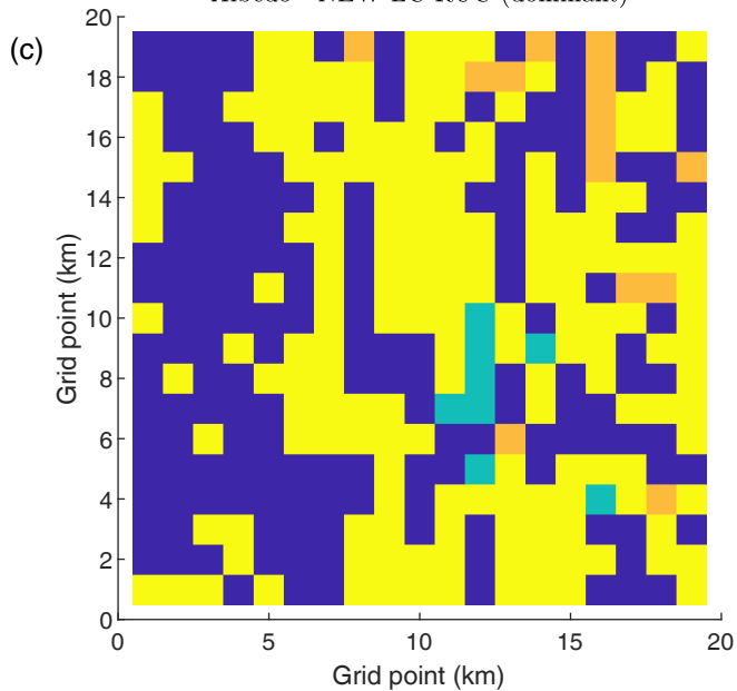
Albedo - NEW-LC-RUC (dominant)
