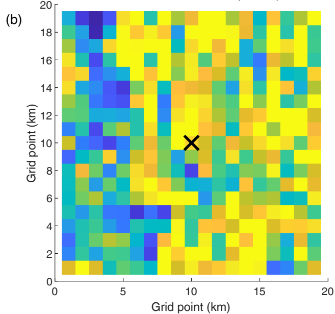
Albedo - MOSAIC-Noah (mosaic)
