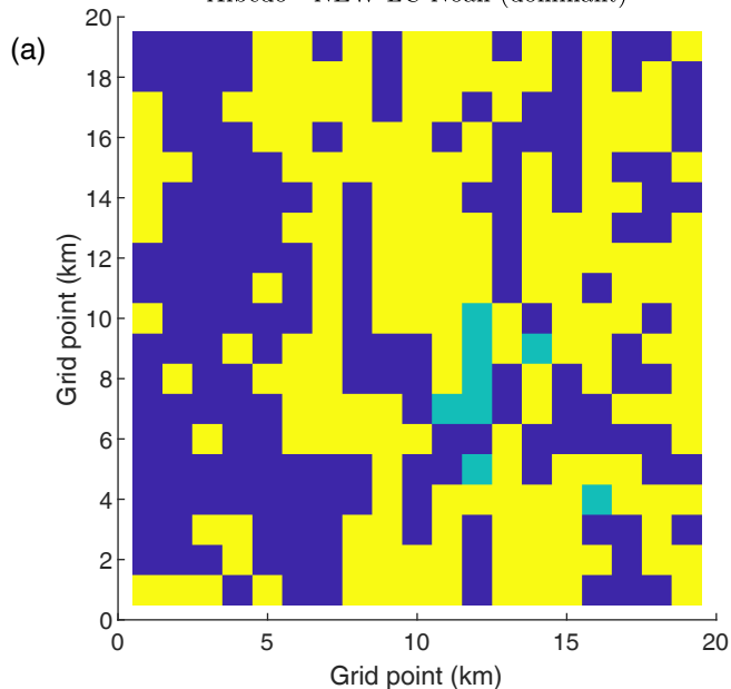
Albedo - NEW-LC-Noah (dominant)
