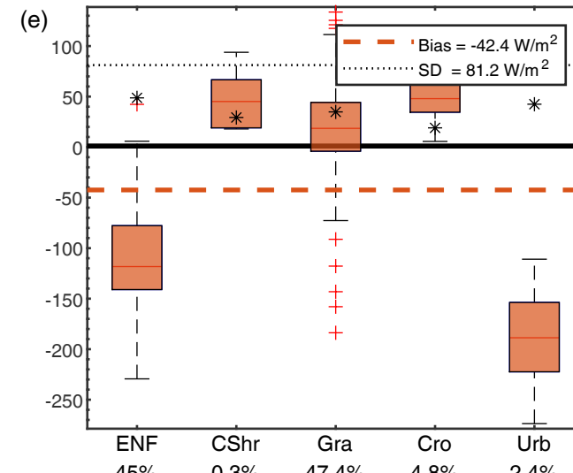
Le bias and its standard deviation NEW-LC-Noah-MP
