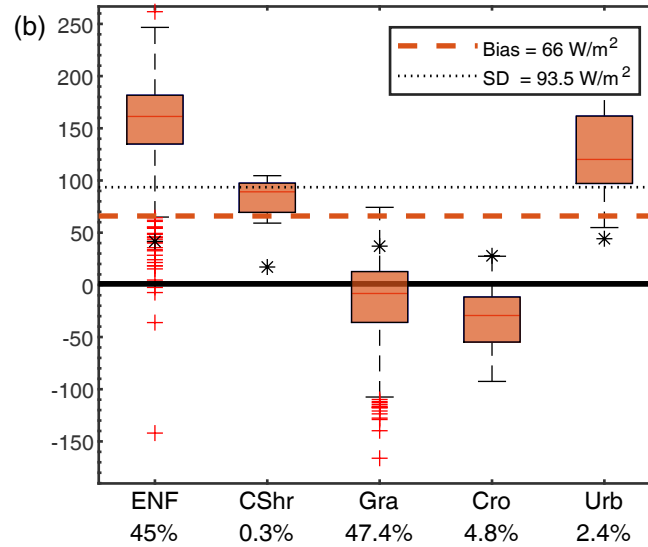
SH bias and its standard deviation NEW-LC-Noah-MP
