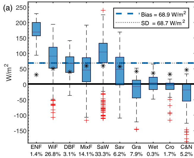
SH bias and its standard deviation DEFAULT-Noah-MP
