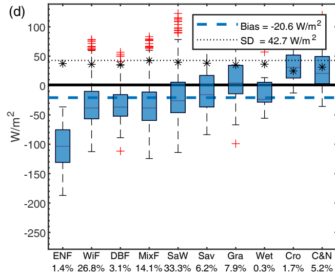
Le bias and its standard deviation DEFAULT-Noah-MP
