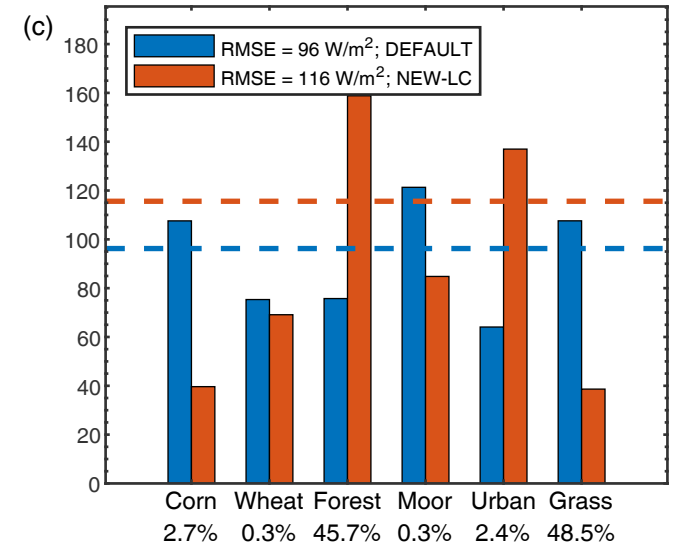
SH RMSE Comparison
