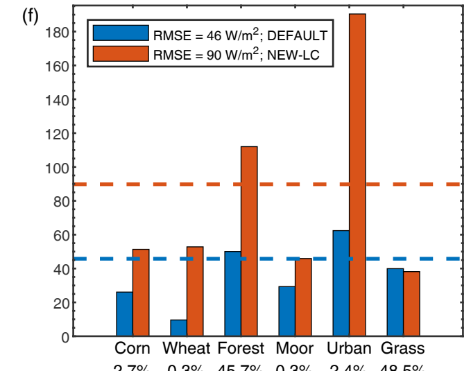
Le RMSE Comparison
