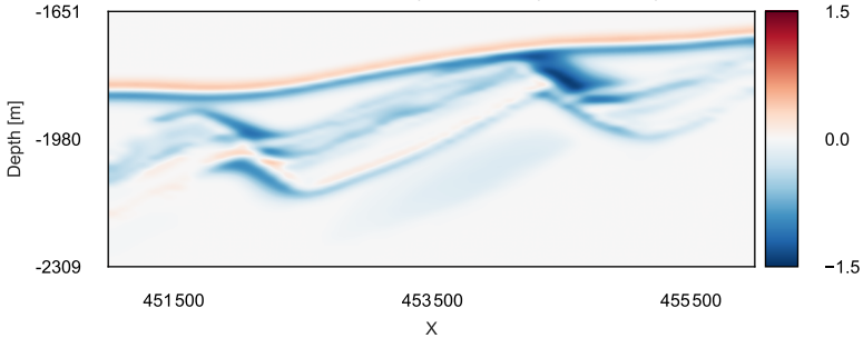
Information Entropy Difference (X-Z Section)
