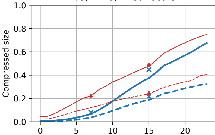
(e) lzma, linear scale
