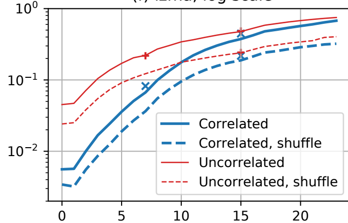
(f) lzma, log scale
