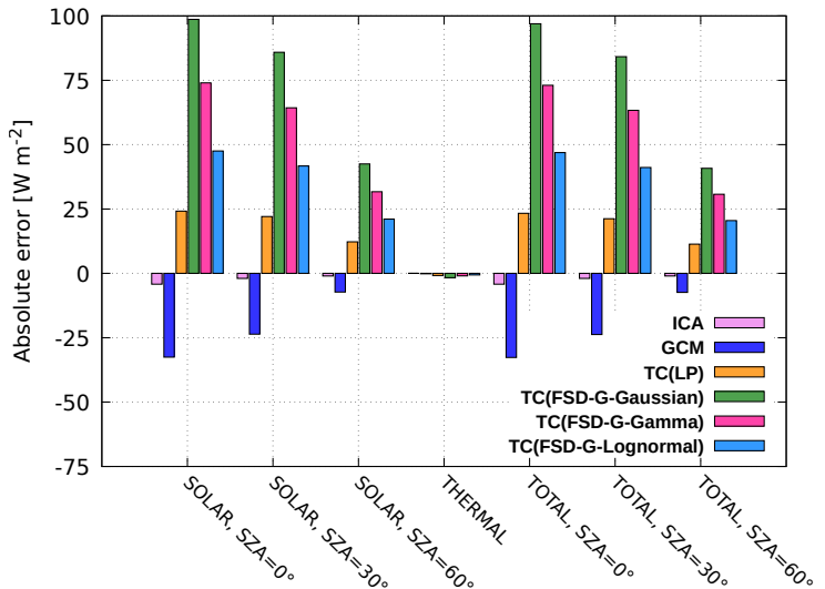
Stratocumulus
