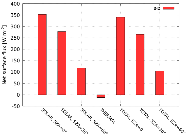
Stratocumulus
