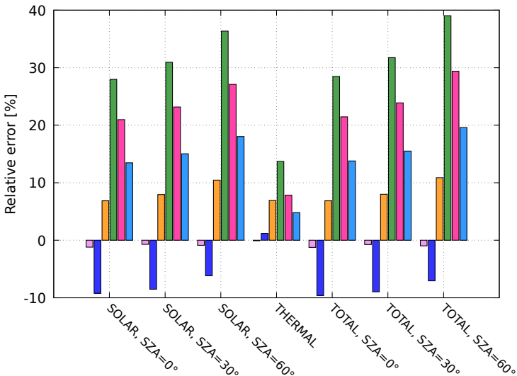
Stratocumulus
