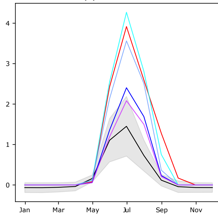
(e) Shrubs GPP
