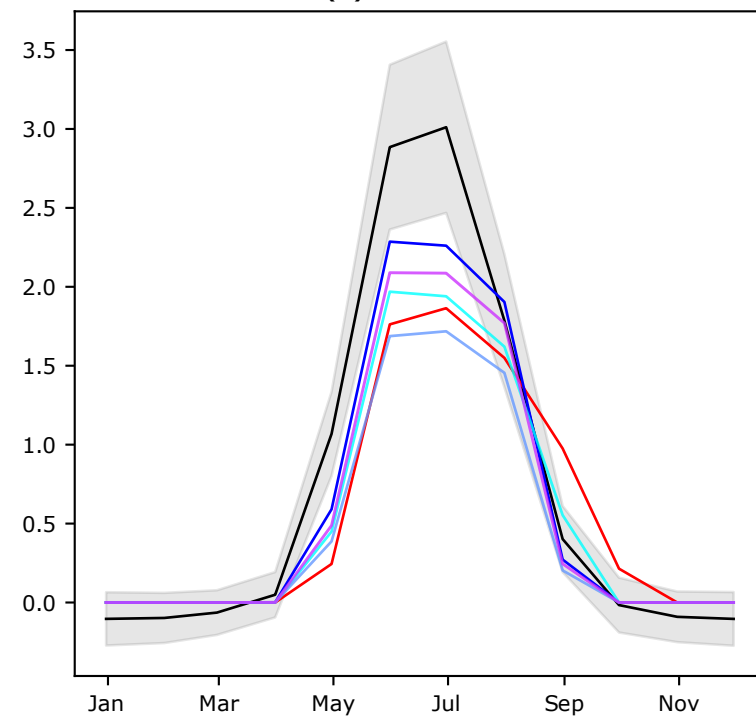
(f) Grasses GPP
