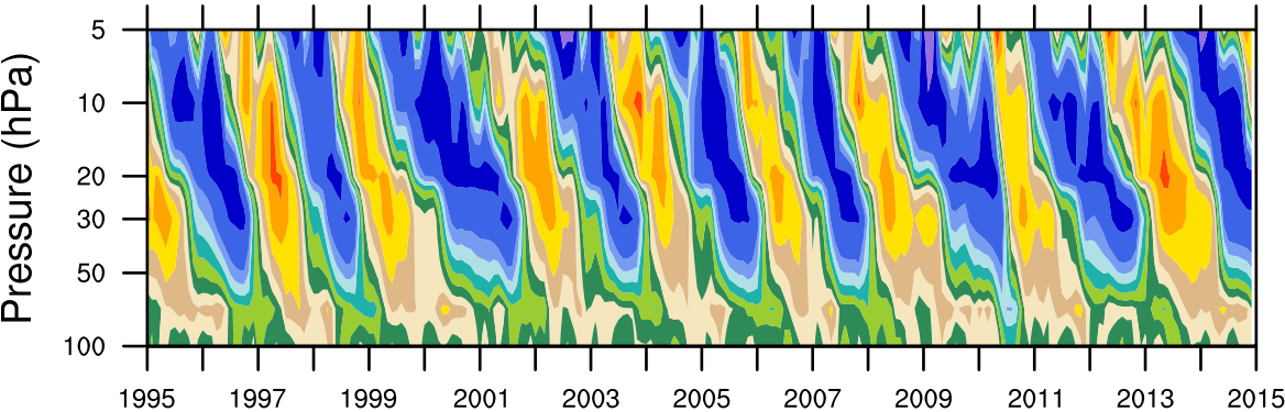
(a) ERA5
