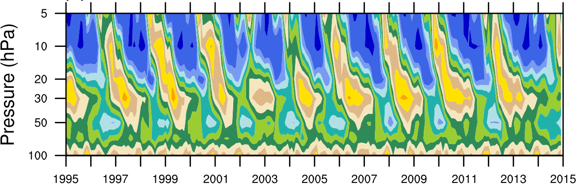
(b) BCC-CSM2-MR
