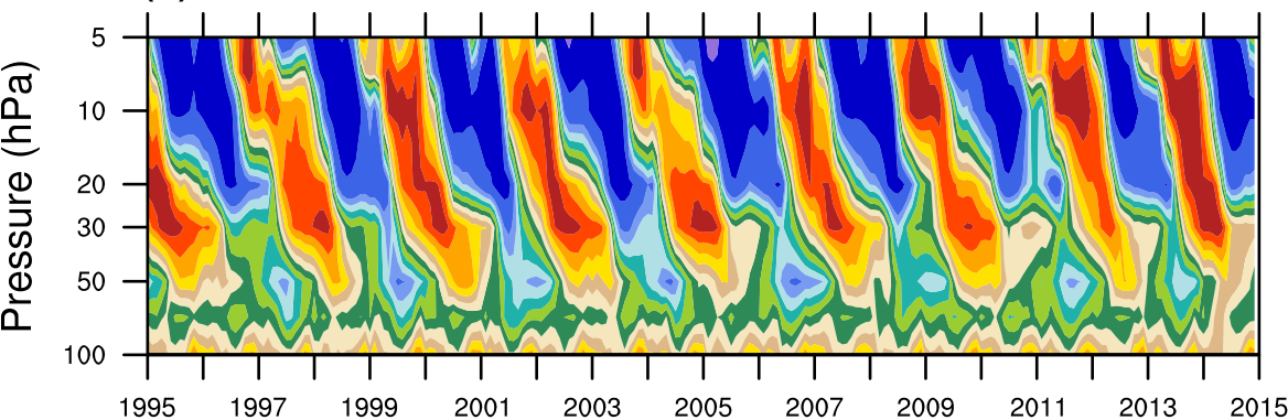
(c) BCC-CSM2-HR
