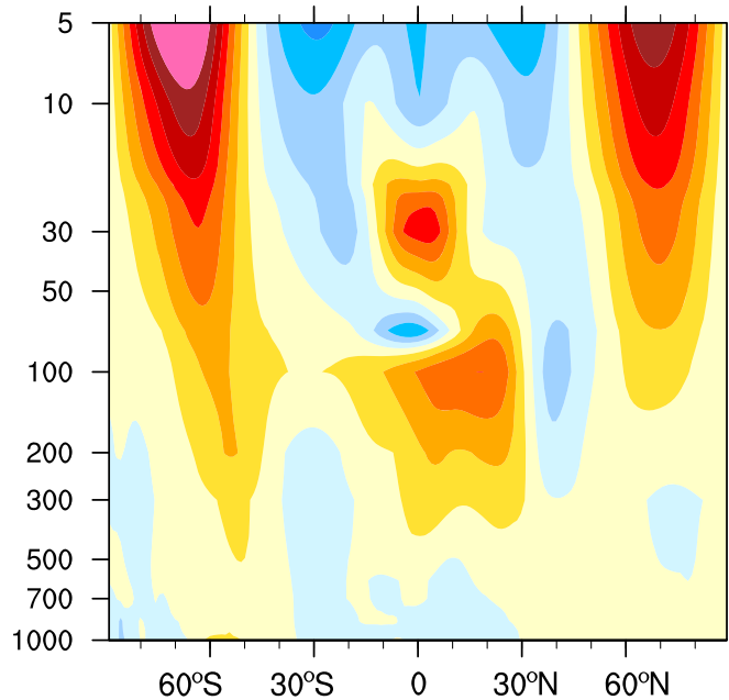
(b) BCC-CSM2-MR minus ERA5 U
