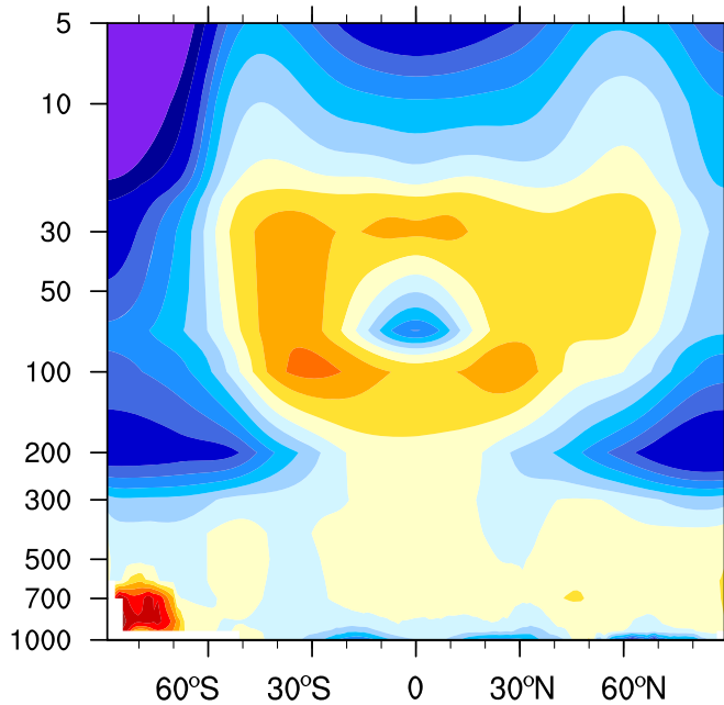
(c) BCC-CSM2-HR minus ERA5 T
