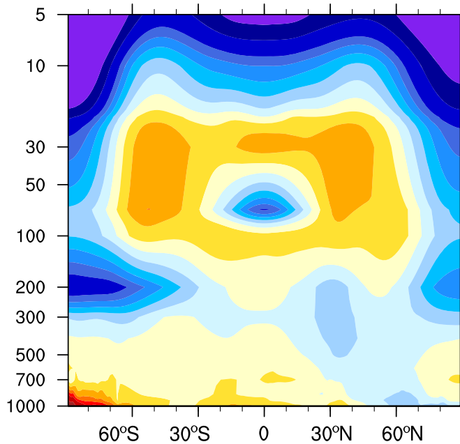
(a) BCC-CSM2-MR minus ERA5 T
