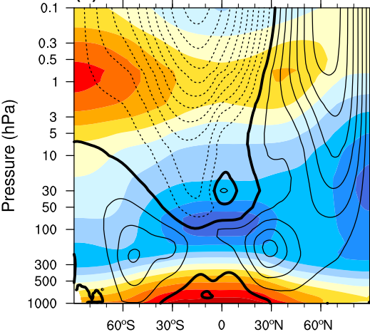
(e) BCC-CSM2-HR
