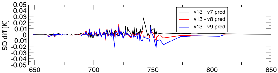
(a) IASI: long-wave temperature sounding region
