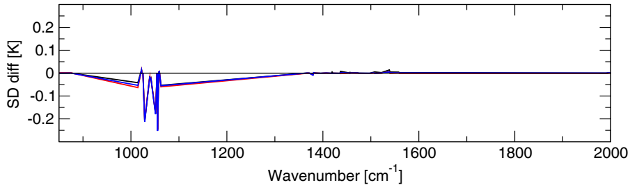
(b) IASI: ozone and water vapour sounding regions
