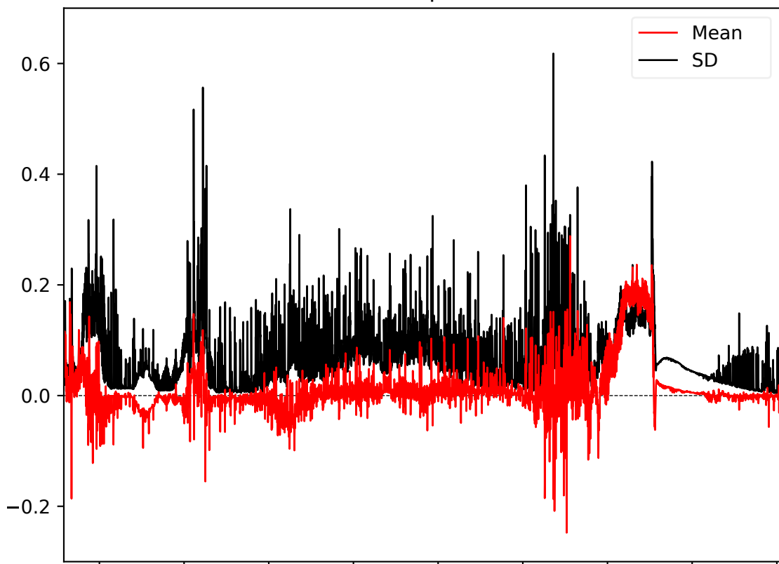
(b) v13pred
