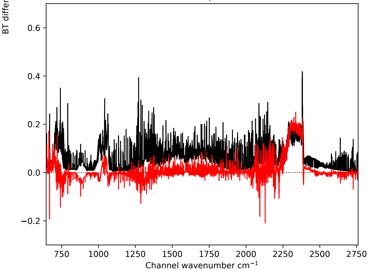
(b) v13pred
