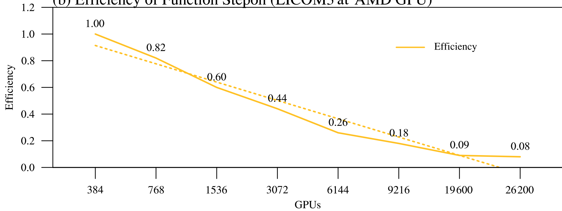
(b) Efficiency of Function Stepon (LICOM3 at AMD GPU)
