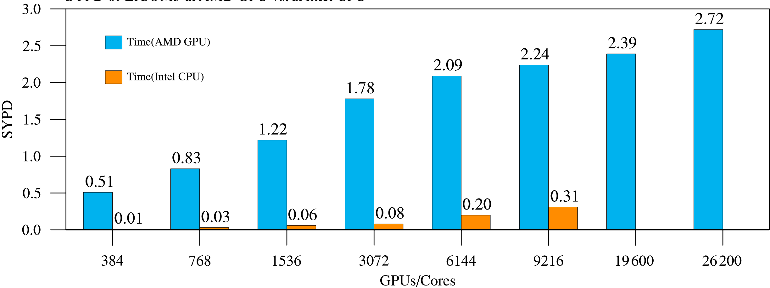
SYPD of LICOM3 at AMD GPU vs. at Intel CPU
