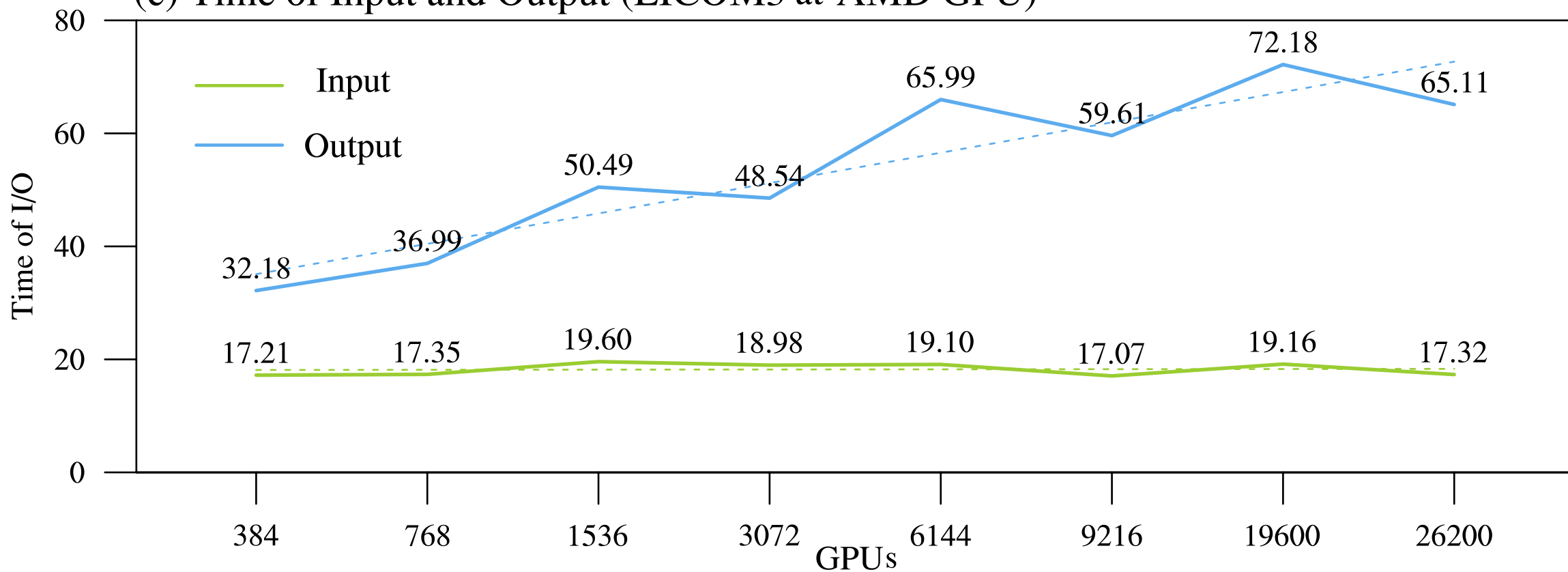
(c) Time of Input and Output (LICOM3 at AMD GPU)
