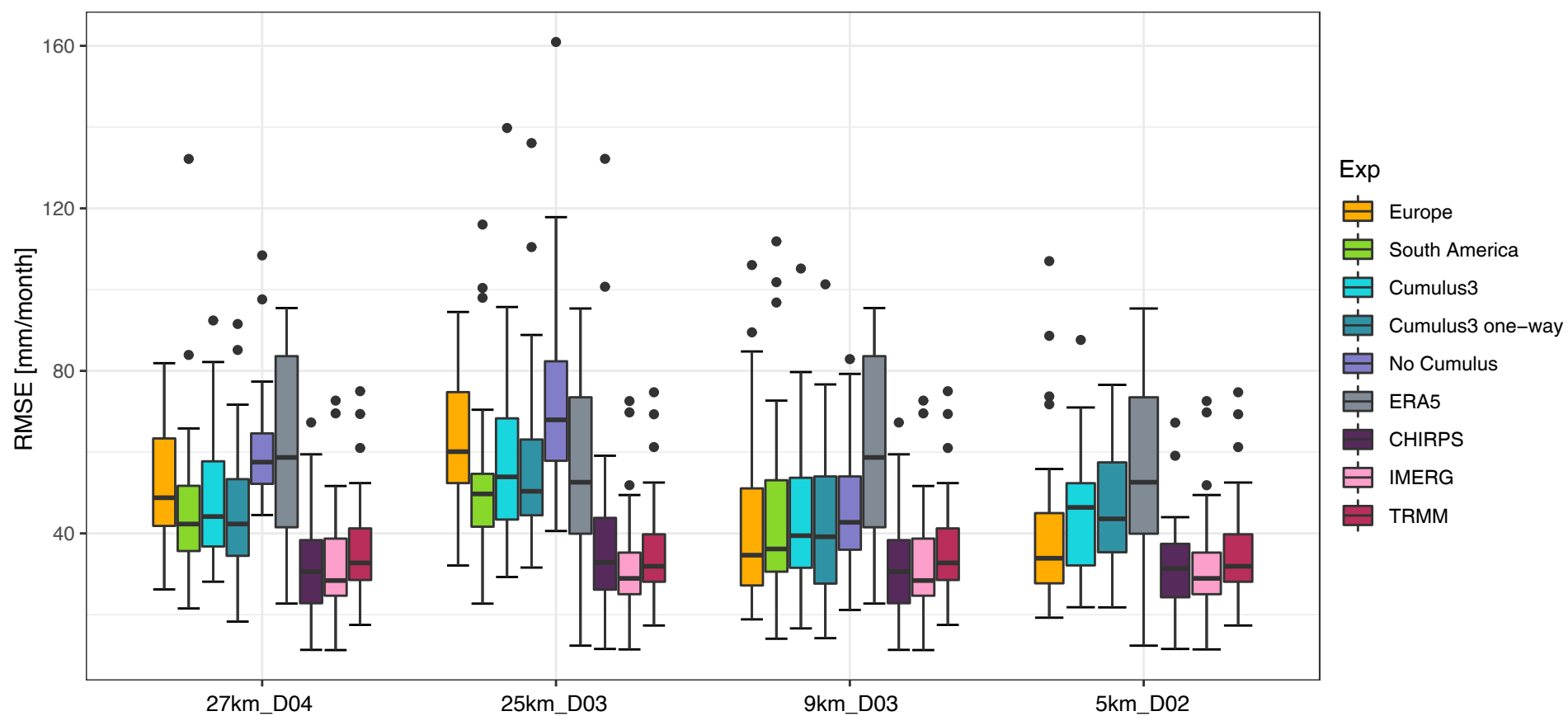
(b) RMSE
