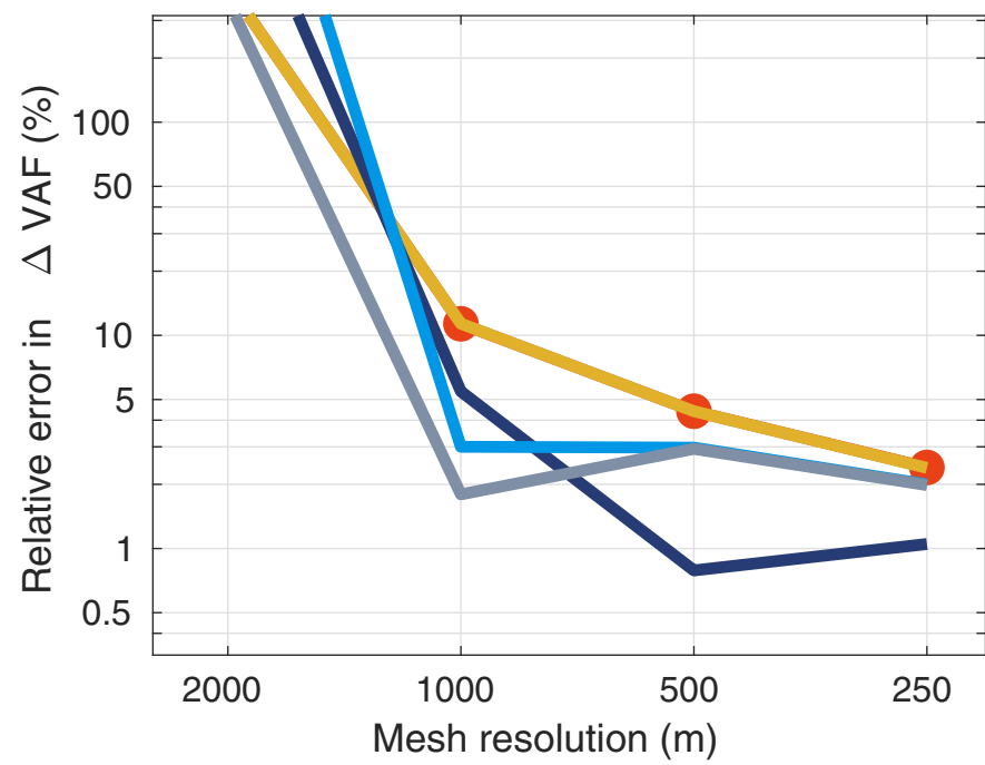
Relative error - SEP1+NSED
