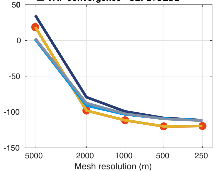
\Delta VAF convergence - SEP2+SED2
