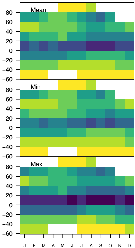
(a) LAI Model Ensemble (N = 6)
