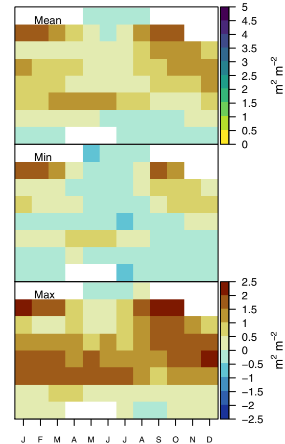
(c) LAI Mean Ensemble Bias (N = 12)
