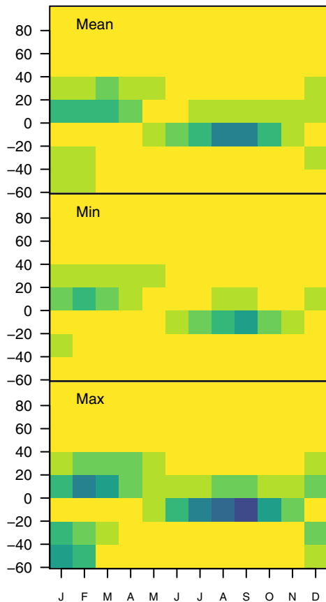
(a) FIRE Model Ensemble (N = 3)
