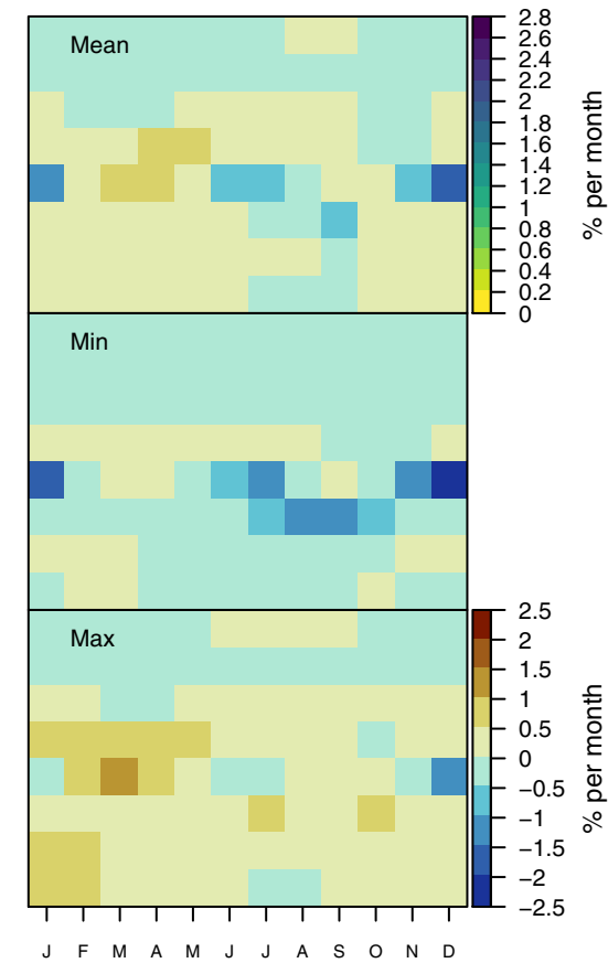
(c) BURNT Mean Ensemble Bias (N = 12)
