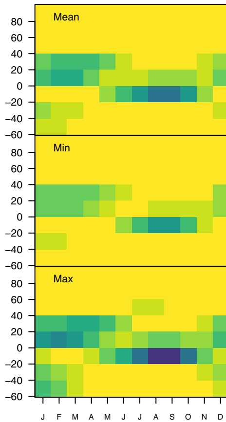
(a) BURNT Model Ensemble (N = 6)
