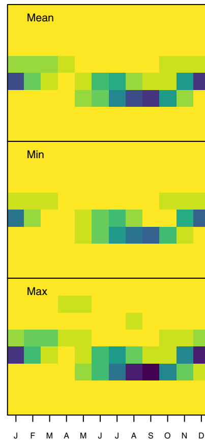
(b) BURNT Reference Ensemble (N = 2)
