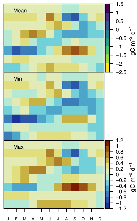
(c) NEE Mean Ensemble Bias (N = 3)
