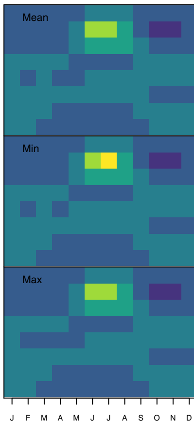
(b) NEE Reference Ensemble (N = 1)
