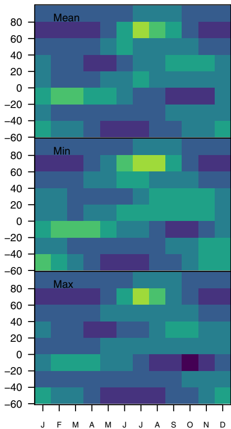
(a) NEE Model Ensemble (N = 3)
