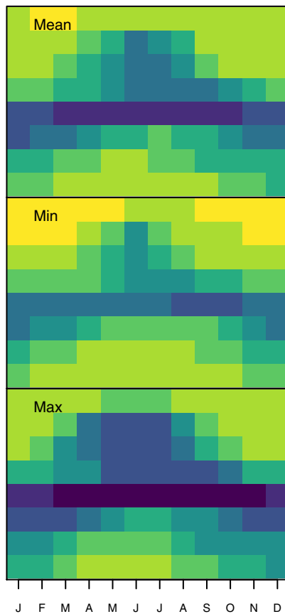
(b) GPP Reference Ensemble (N = 3)
