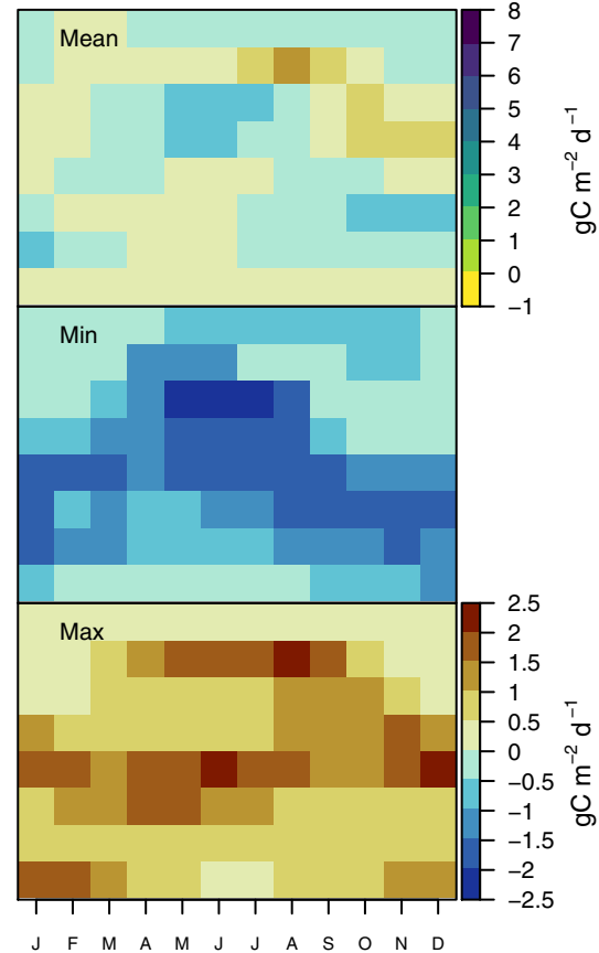
(c) GPP Mean Ensemble Bias (N = 27)
