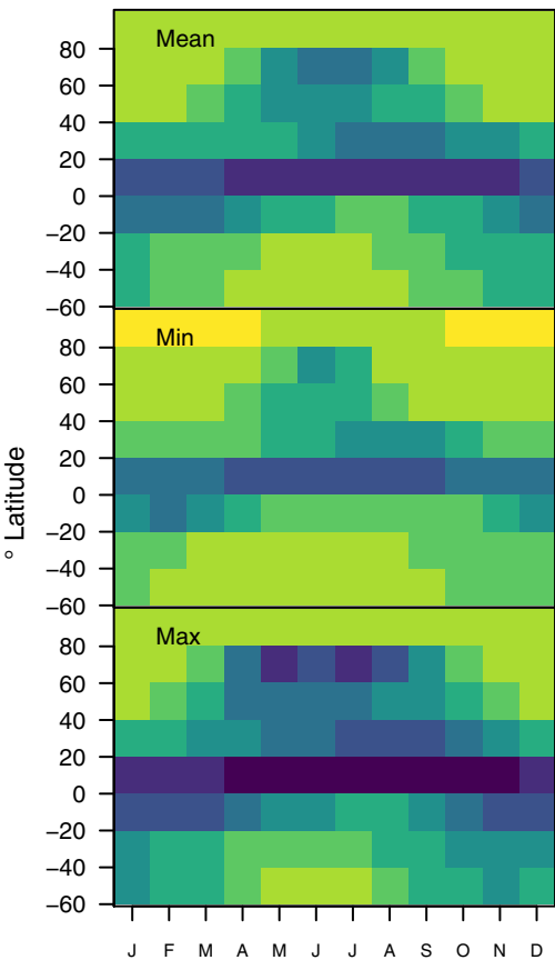
(a) GPP Model Ensemble (N = 9)
