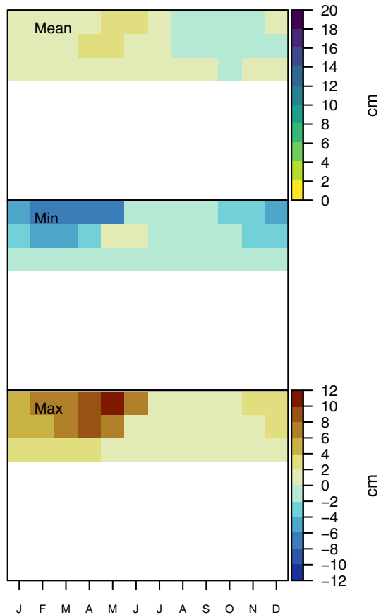
(c) SNW Mean Ensemble Bias (N = 48)
