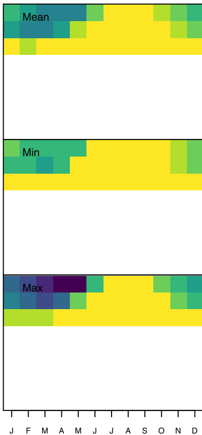
(b) SNW Reference Ensemble (N = 4)
