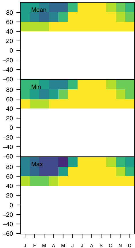
(a) SNW Model Ensemble (N = 12)
