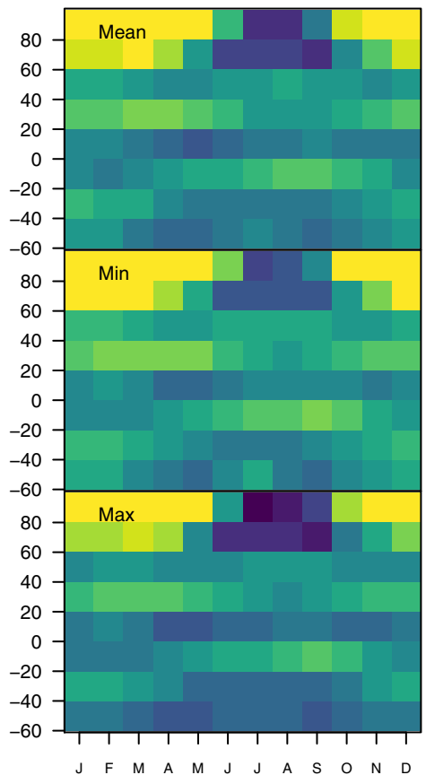
(a) MRSLL Model Ensemble (N = 3)
