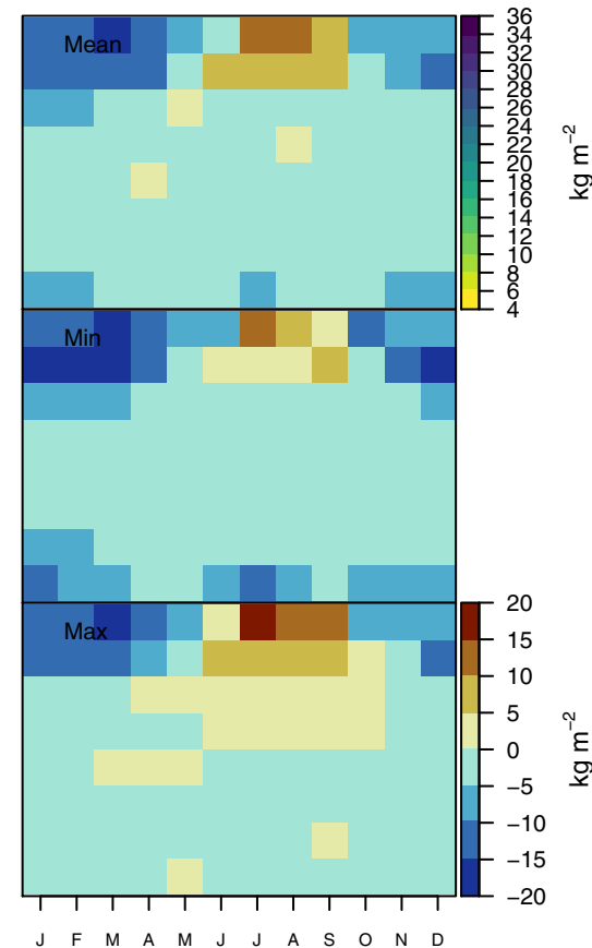
(c) MRSLL Mean Ensemble Bias (N = 3)
