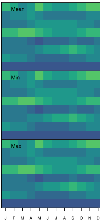
(b) MRSLL Reference Ensemble (N = 1)
